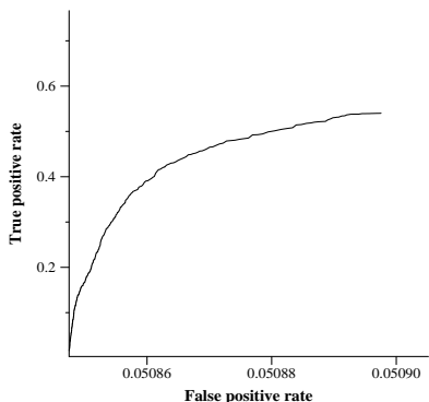
average ROC curve for IBCN4
