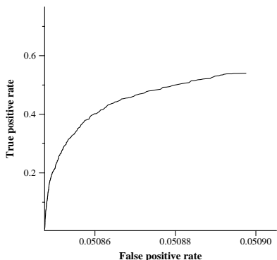
average ROC curve for IBCN3
