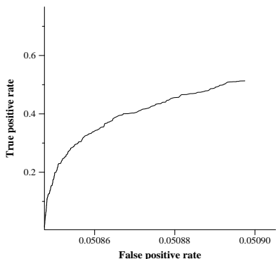
average ROC curve for IBCNI
