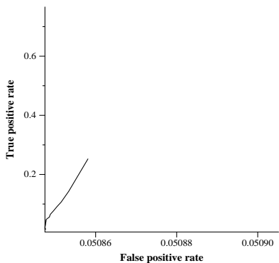
average ROC curve for FASILKOM04
