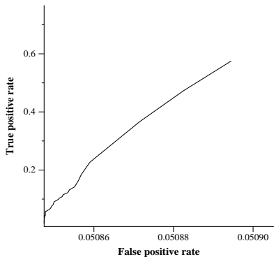
average ROC curve for FASILKOM02
