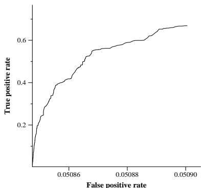
average ROC curve for BAUdph
