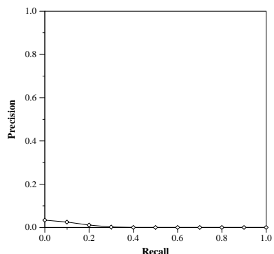
Recall-Precision Curve
