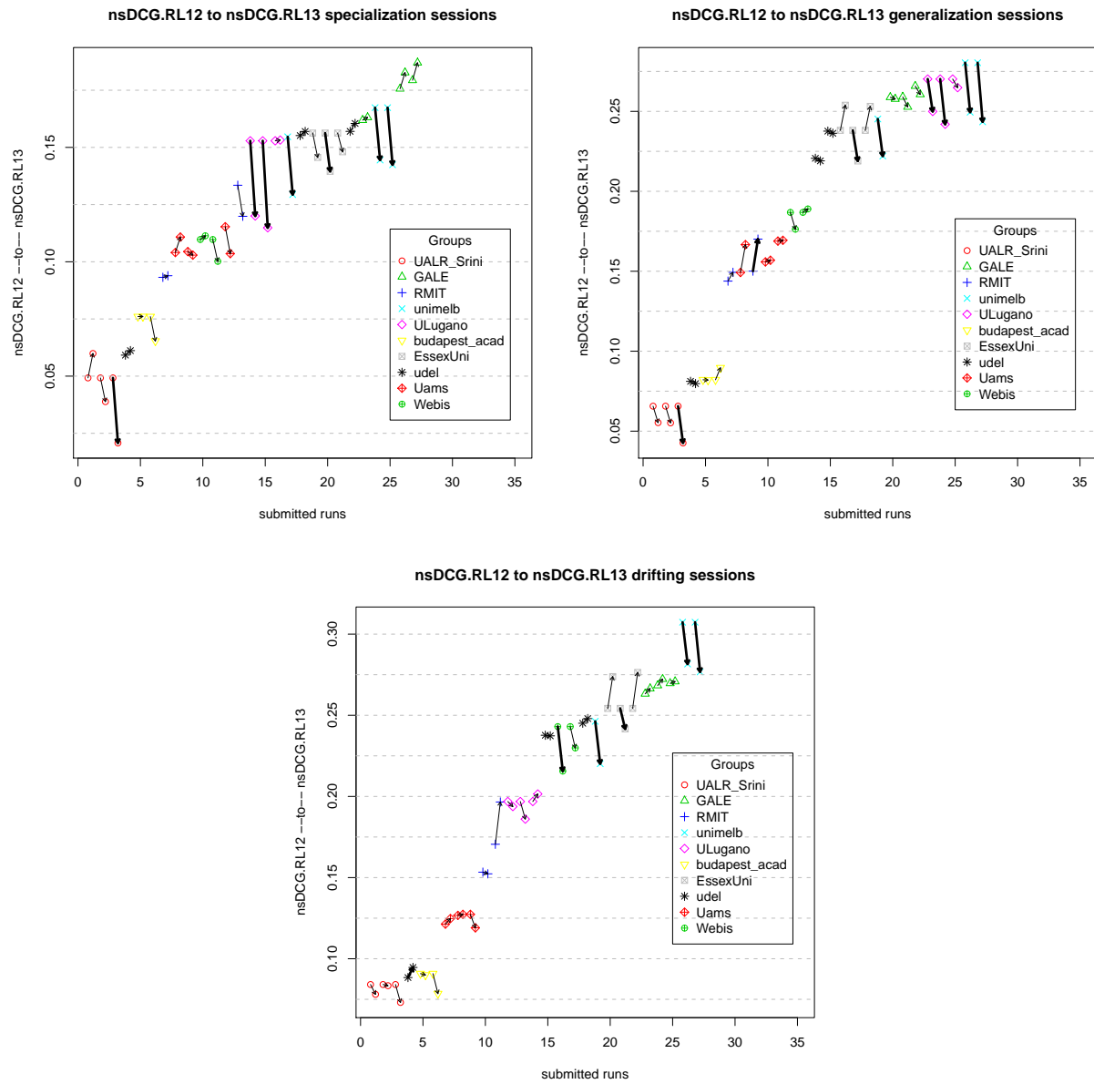
Figure 7: Evaluation scores based on nsDCG@10 for all submitted runs for the ranked lists RL1 \rightarrow RL2 and RL1 \rightarrow RL3 for specification, generalization and drifting-reformulation sessions.
