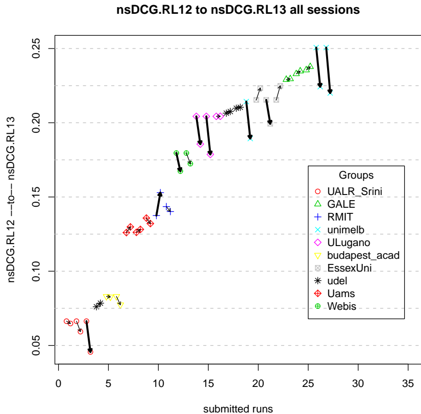
Figure 6: Evaluation scores based on nsDCG@10 for all submitted runs for the ranked lists RL1 → RL2 and RL1 → RL3. Arrows indicate the change in the evaluations score between the two ranked lists for each one of the submitted runs. Thick solid arrows indicate statistically significant changes according to paired two-sided Student t-test.
