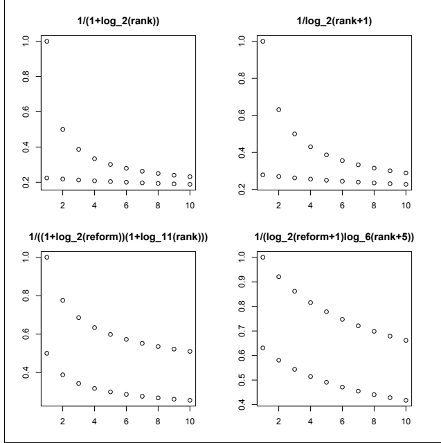
Figure 5: Different discounts for top 10 documents in the first query and the query reformulation. The discounts are shown for the two queries in isolation, starting from rank 1 in both cases.
