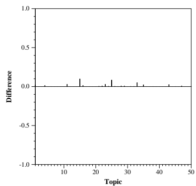
Difference from median statAP per topic
