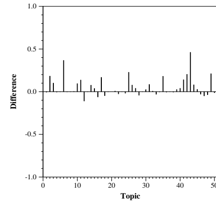
MAP Per Topic Median Diff, WAT2.WatS.2
