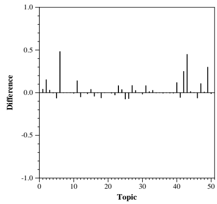
MAP Per Topic Median Diff, WAT2.udel.1
