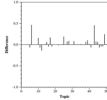
MAP Per Topic Median Diff, WAT2.UCSC.1
