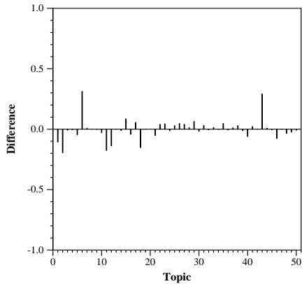
MAP Per Topic Median Diff, WAT2.base
