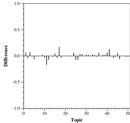
MAP Per Topic Median Diff, WAT2.CMIC.2
