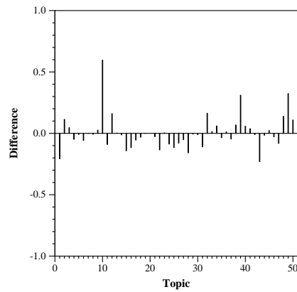
statAP Per Topic Median Diff, CMIC.ugTr.2
