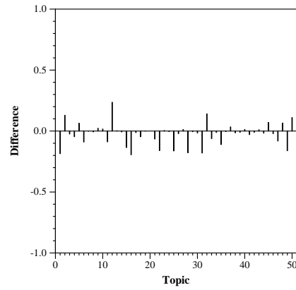
statAP Per Topic Median Diff, CMIC.udel.2
