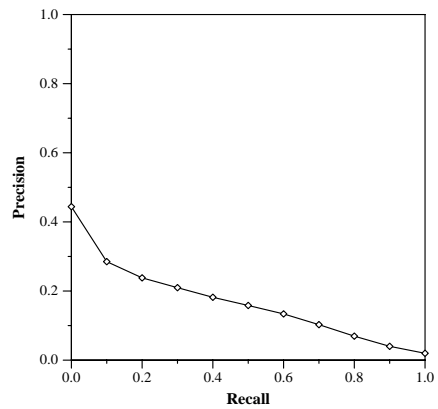
Recall-Precision Curve
