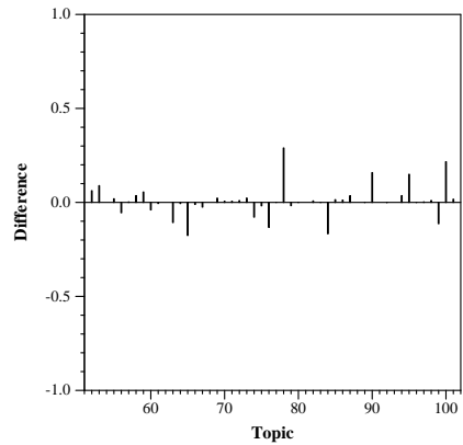
Difference from median est_RB per topic among automatic runs
