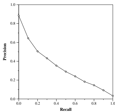
Recall-Precision Curve
