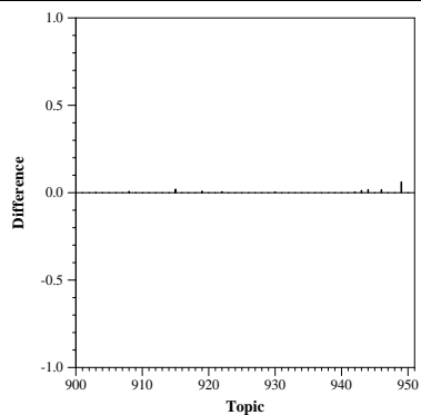
Difference from Median R-accuracy per Topic
