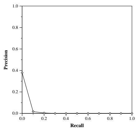
Recall-Precision Curve
