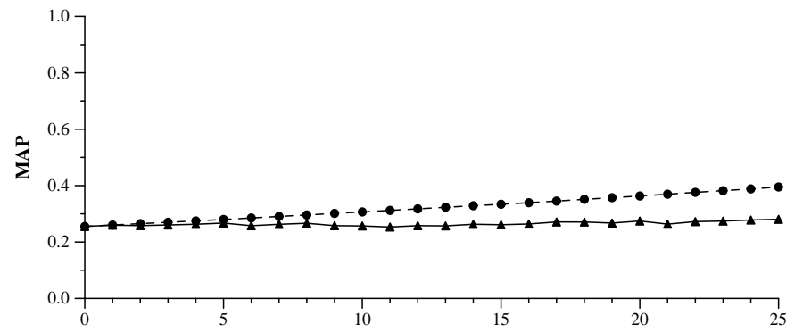
Area between optimal and predicted MAP curves: 1.4923
