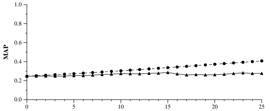
Area between optimal and predicted MAP curves: 1.4966
