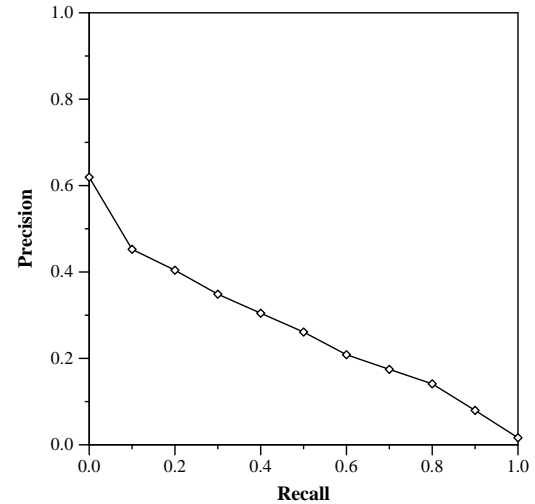
Recall-Precision Curve
