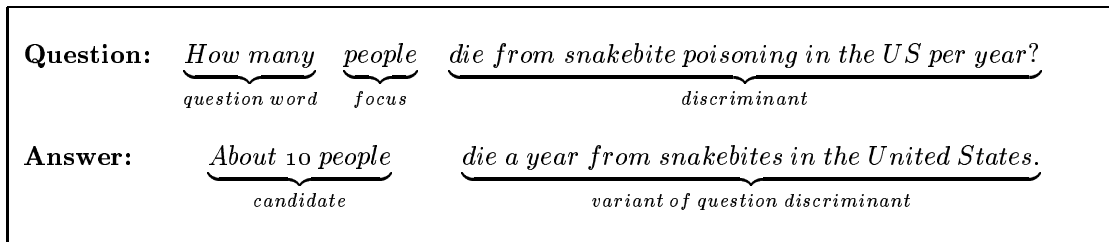
Figure 1: Example of question and answer decomposition. The question is from TREC-9 (# 302) and the answer is from the TREC text collection (document LA082390-0001).
