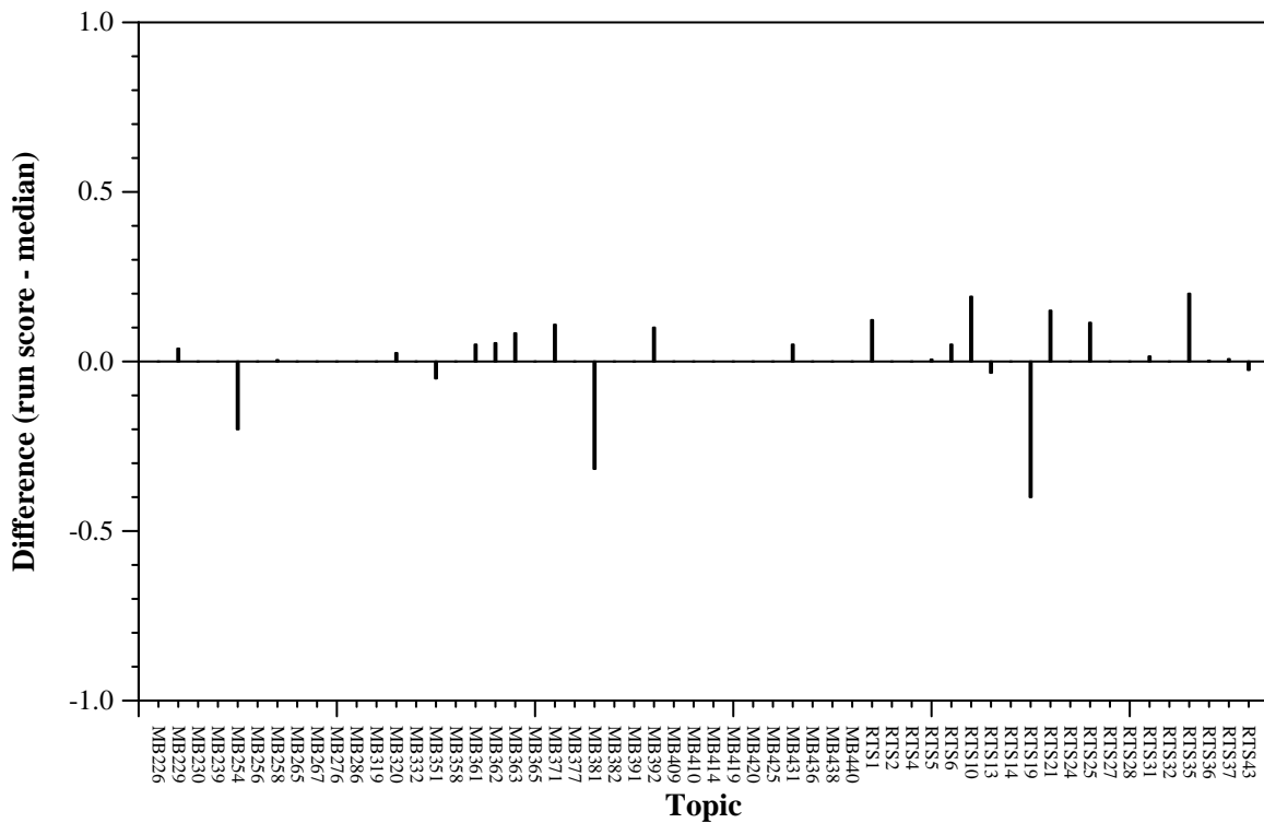
Per-topic difference from median ELG-1
