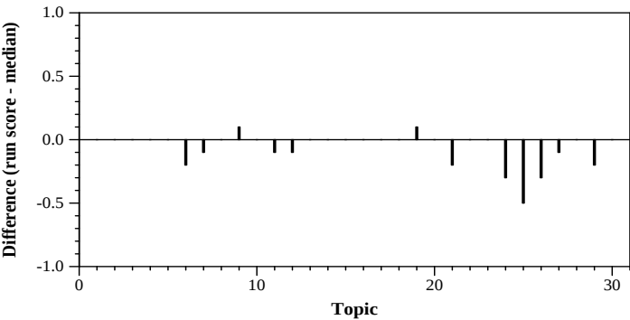
Per-topic difference from median P@10 for Automatic, Note runs
