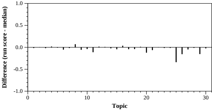
Per-topic difference from median infNDCG for Automatic, Note runs
