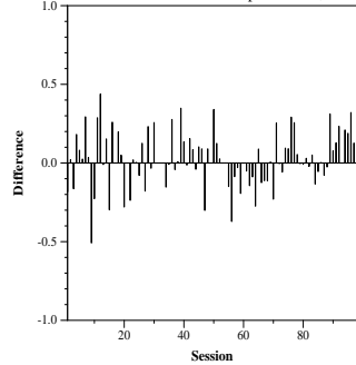
Difference from median nDCG per session, run RL4
