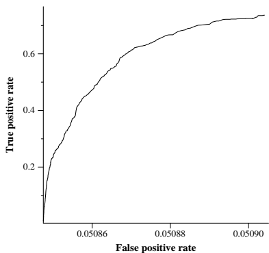
average ROC curve for york12mb4
