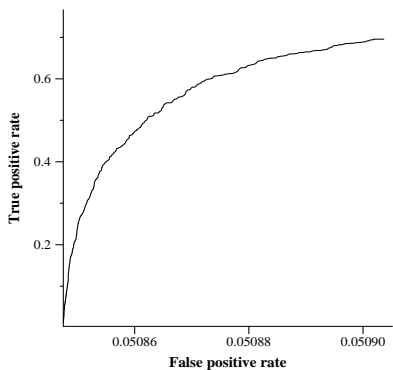
average ROC curve for urlContent
