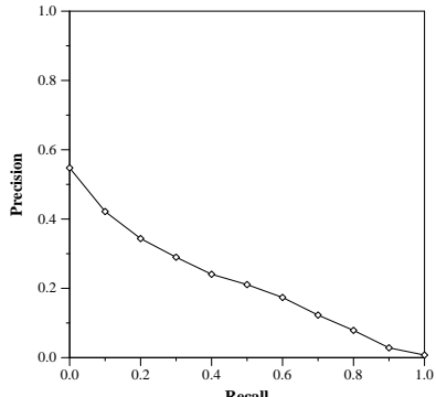
Recall-Precision Curve
