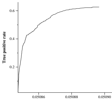
average ROC curve for kobeL2R
