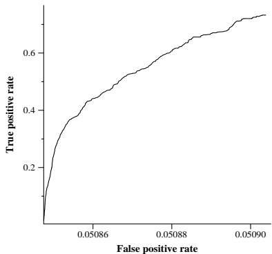
average ROC curve for hitLRrun1
