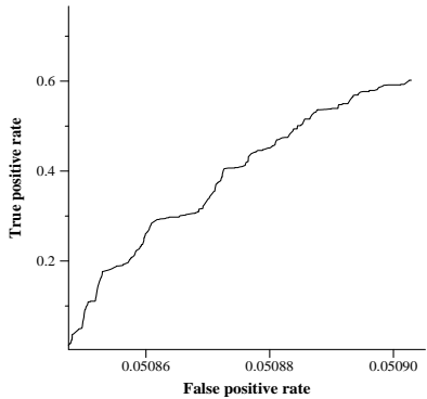
average ROC curve for csiroQEt112
