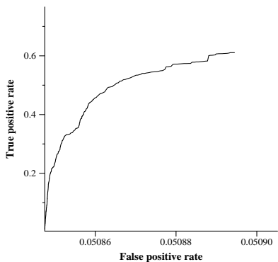
average ROC curve for XMRUN4
