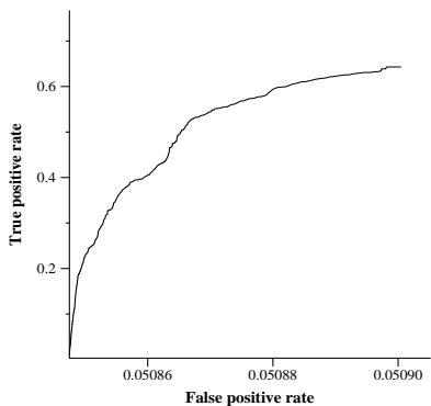
average ROC curve for XMRUN2
