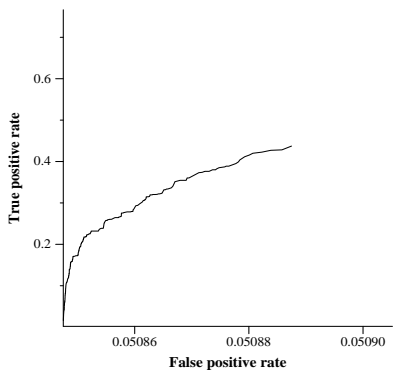
average ROC curve for UvAfilter
