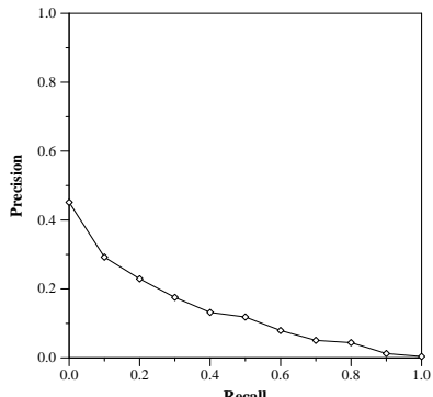
Recall-Precision Curve
