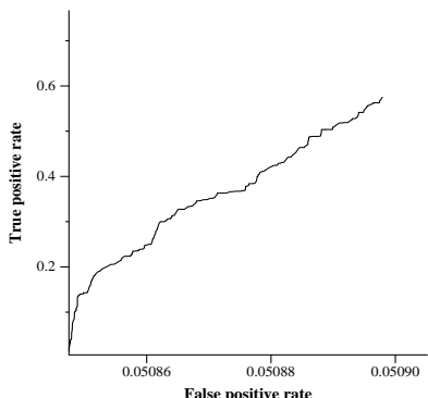
average ROC curve for UNCTP
