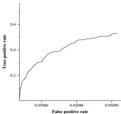
average ROC curve for UDInfoMBCW
