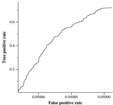
average ROC curve for QWebFB
