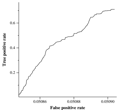
average ROC curve for QEWeb
