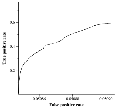
average ROC curve for PKUICST2
