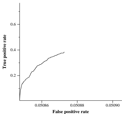
average ROC curve for IRITfdvsmurl
