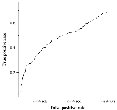
average ROC curve for IBMBaseline
