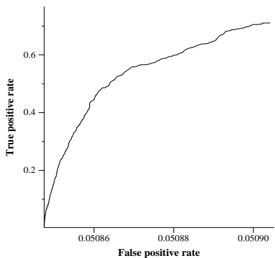
average ROC curve for BM25TRF
