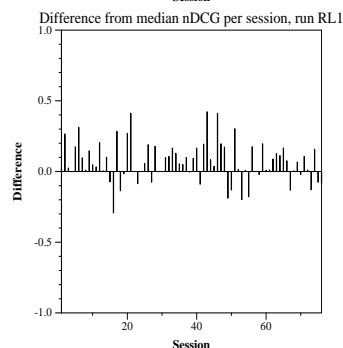
Difference from median nDCG per session, run RL1
