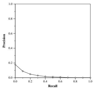
Recall-Precision Curve
