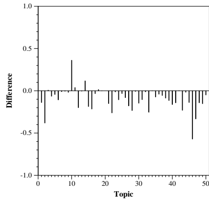
statAP Per Topic Median Diff, QUT.UPD.1
