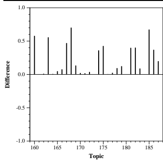
Difference from median document AP per topic among automatic runs
