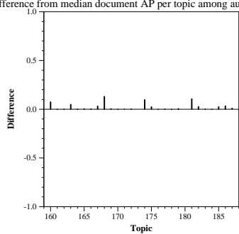
Difference from median passage AP per topic among automatic runs
