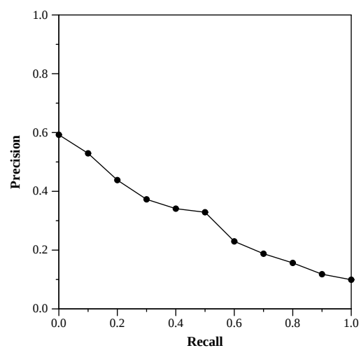
Recall-precision graph for document ranking task
